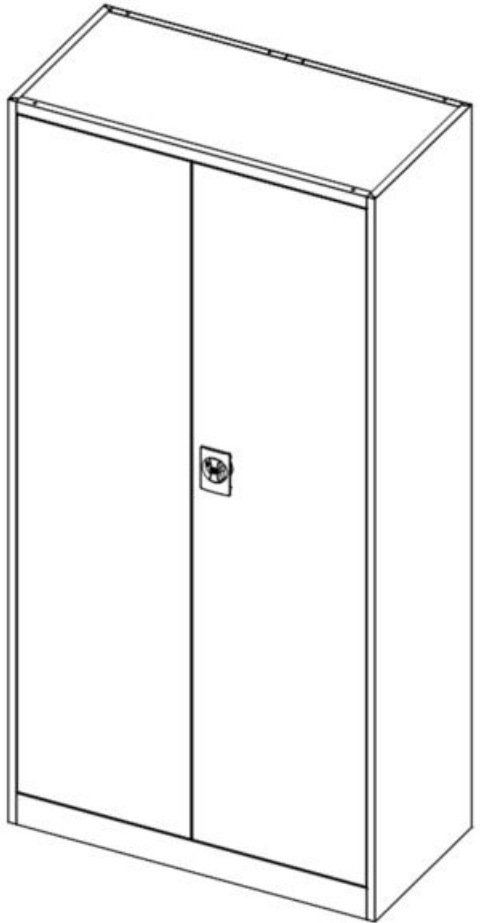
STEEL 2-SWING DOOR STORAGE CABINET (STRUCTURE: SPLIT BACK PANEL STRUCTURE) PRODUCT SIZE: H1850*W900*400MM
